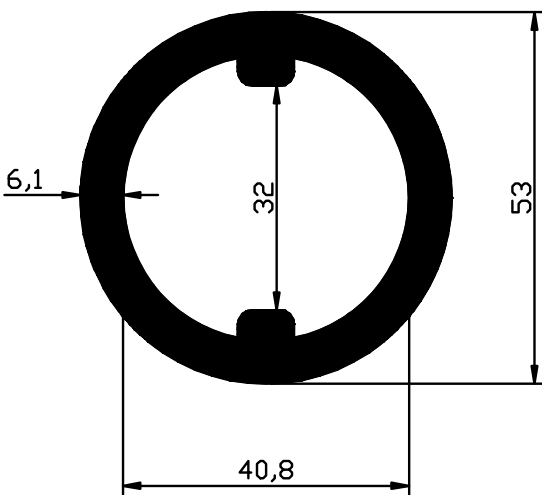
2180 - 2.612 Kg/m
