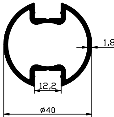
1869 - 0.755 Kg/m
