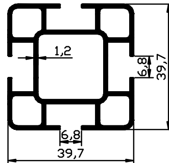
1971 0.990 Kg/m
