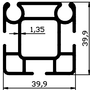
1966 0.995 Kg/m
