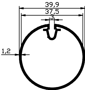
1964 - 0.447 Kg/m
